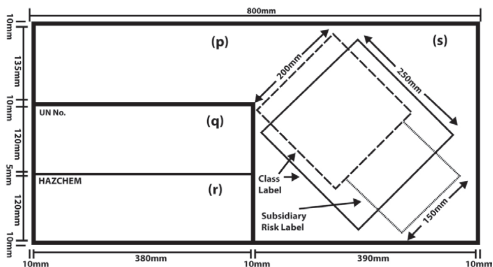
Figure 13.2 Template for a placard for a hazardous chemical stored in bulk
